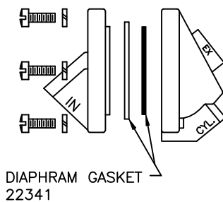
QUICK EXHAUST VALVE 17799
