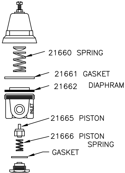
1/4"REGULATOR 16048
