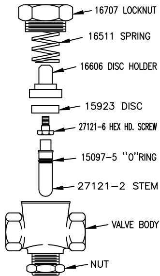
1/4" AIR WHISTLE VALVE 15100
