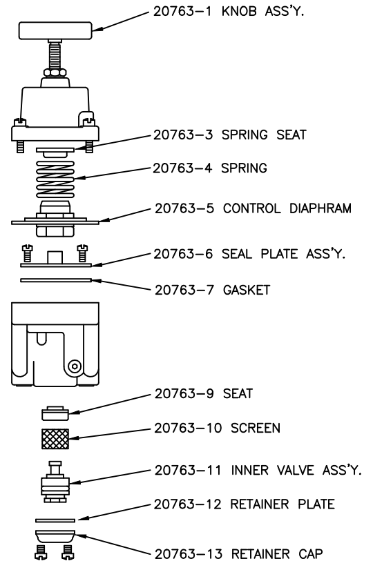
3/8"PRECISION REGULATOR 20763
