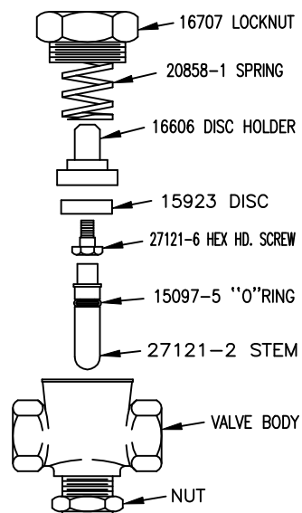
1/4" AIR WHISTLE VALVE WEAKER SPRING 20858
